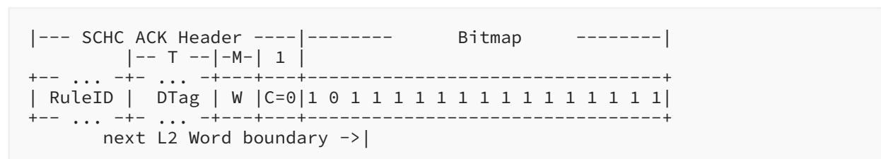
Figure 16: SCHC ACK Header Plus Uncompressed Bitmap
