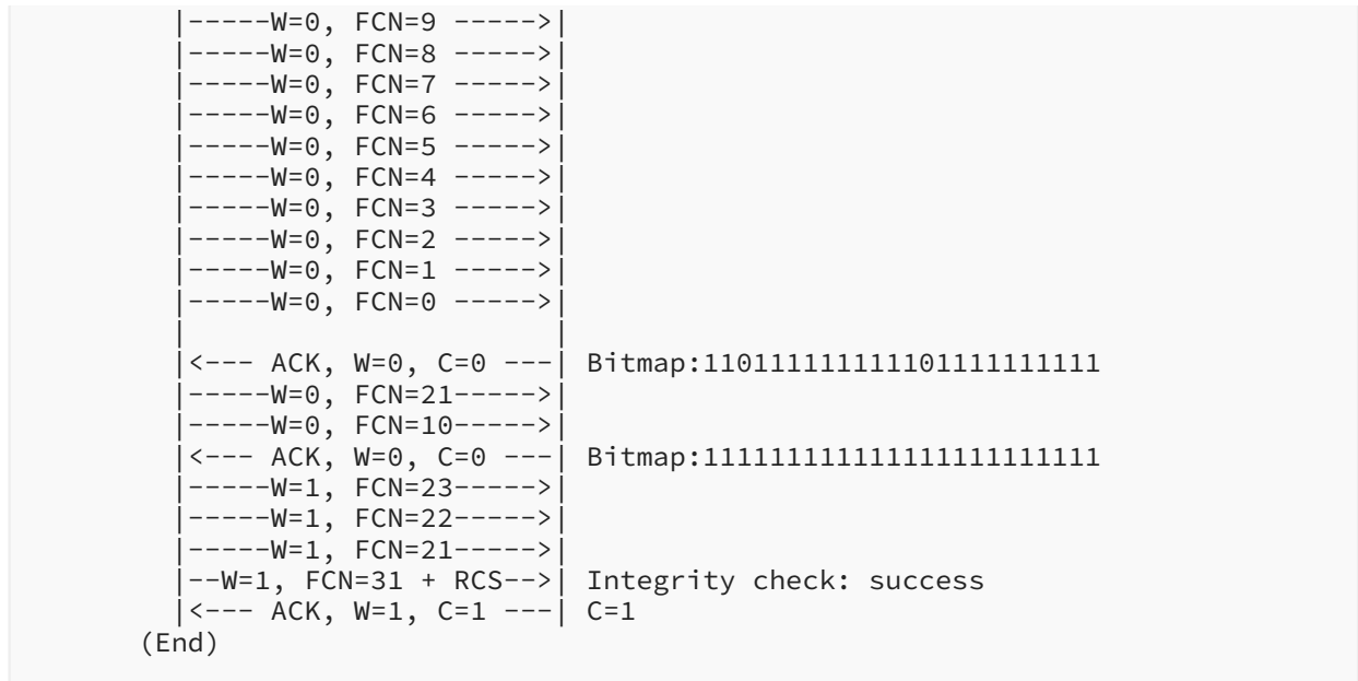
Figure 38: ACK-Always Mode, 28 Tiles, One Tile per SCHC Fragment, Lost SCHC Fragments
