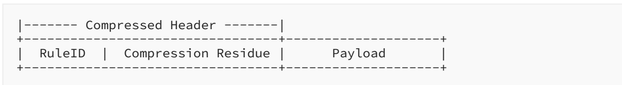
Figure 4: SCHC Packet
