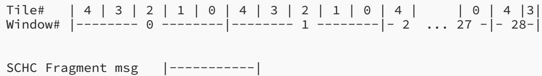
Figure 23: SCHC Packet Fragmented in Tiles, ACK-on-Error Mode
