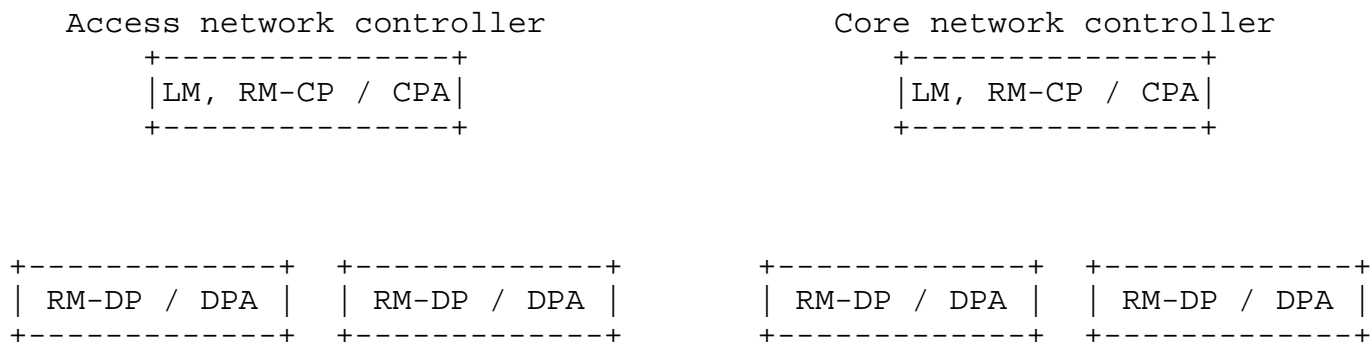
Figure 2: Mobility management functions with data plane - control plane separation with separate control in core and in access.
