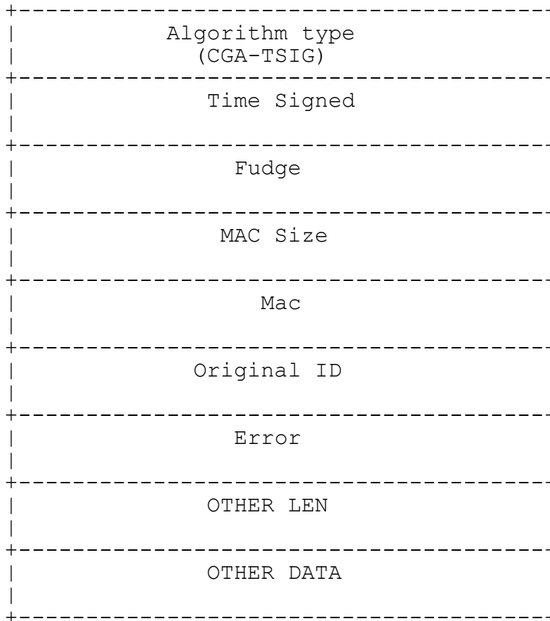
Figure 3 Modified TSIG RDATA
