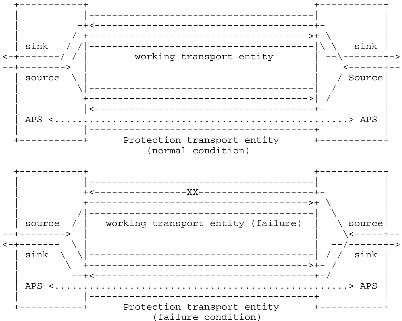
Figure 2: 1+1 bidirectional linear protection switching
